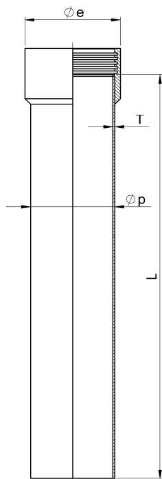
TUBO SCARPA / SHOE PIPE
