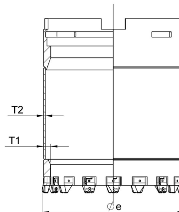
TUBO SCARPA / SHOE PIPE
